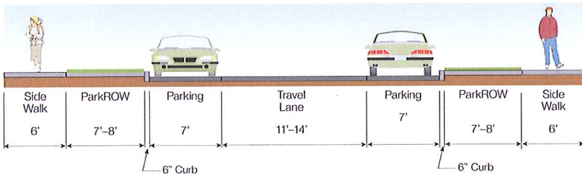
Neighborhood Street (Parking on Both Sides) ROW 50' - 57'
